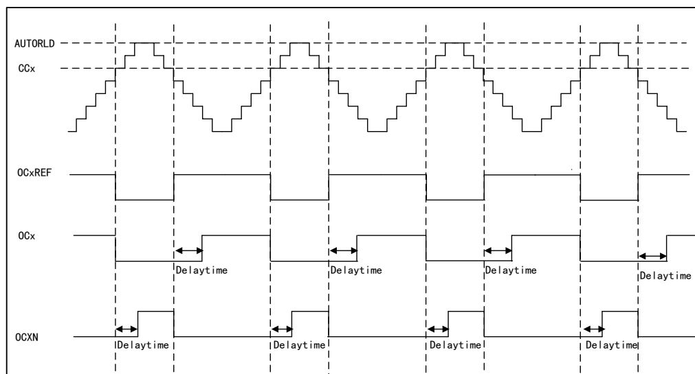
Figure 36 Complementary Output of Insertion with Dead Zone
