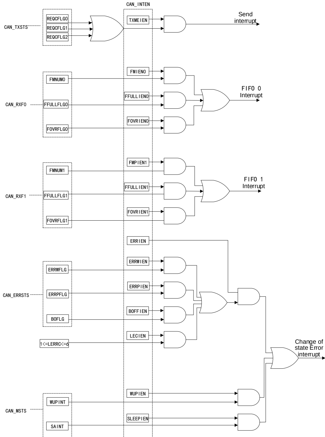
Figure 109 Event Flag and Interrupt Generation
