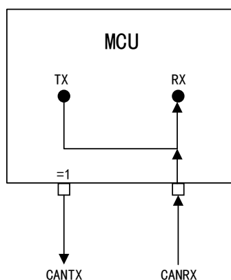
Figure 103 CAN Works in Silent Mode
