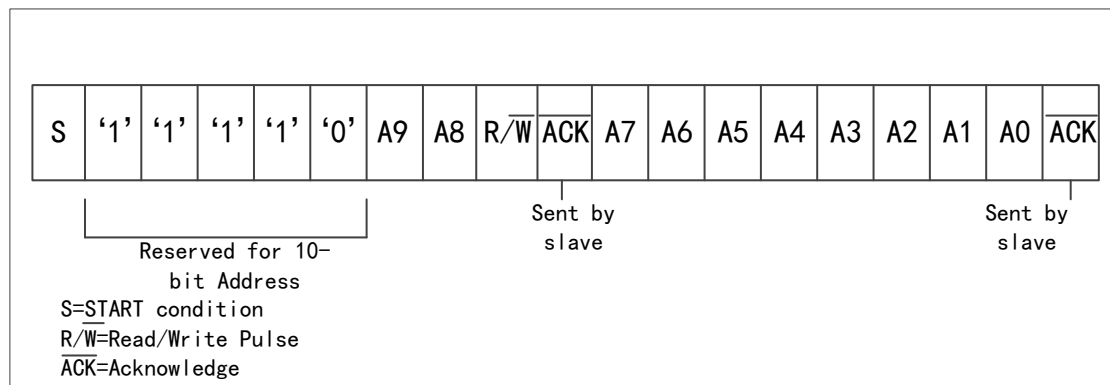
Figure 83 10-bit Address Format
