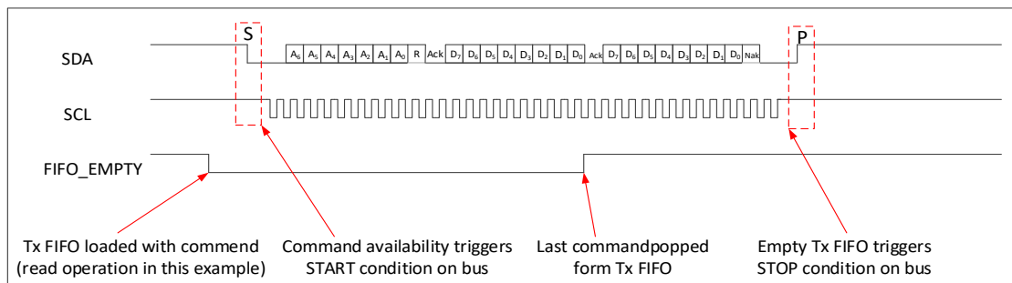
Figure 87 I2C Timing Diagram "Taking TXFIFO as Master Receiver"
