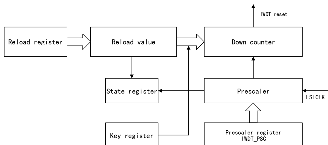
Figure 58 Independent Watchdog Structure Block Diagram
