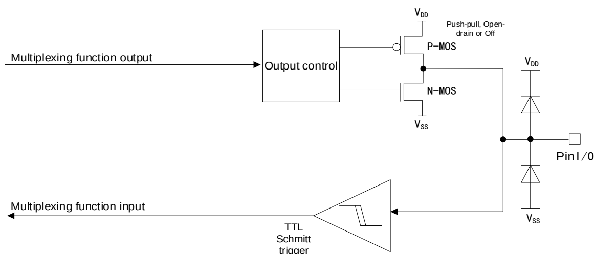
Figure 20 I/O Structure in Multiplexing Mode
