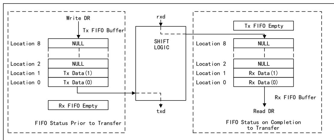
Figure 94 QSPI Transmit FIFO State in Transmitting and Receiving State
