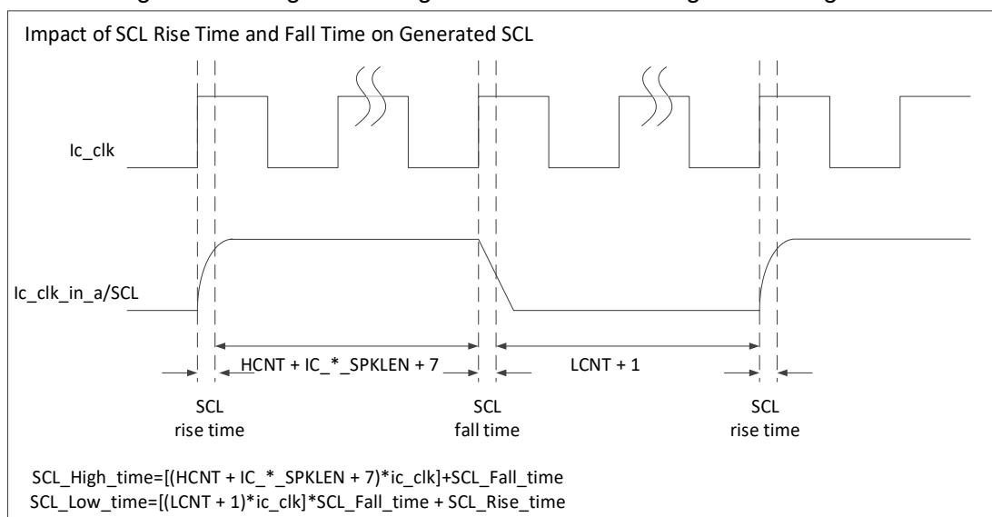
Figure 89 Rising and Falling Time Parameter Configuration Diagram
