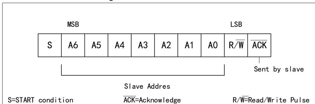
Figure 82 7-bit Address Format
