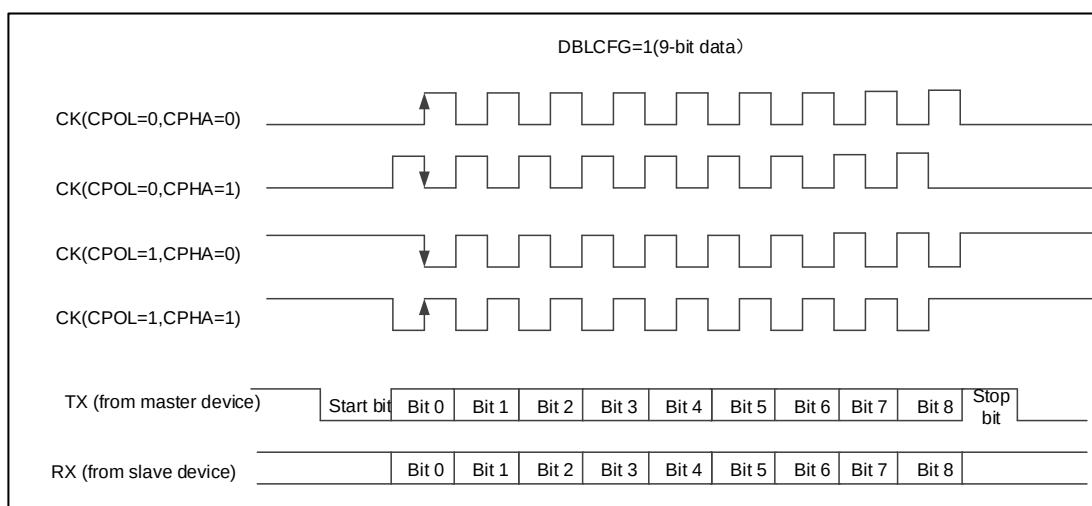
Figure 66 USART Synchronous Transmission Timing Diagram (DBLCFG=1)
