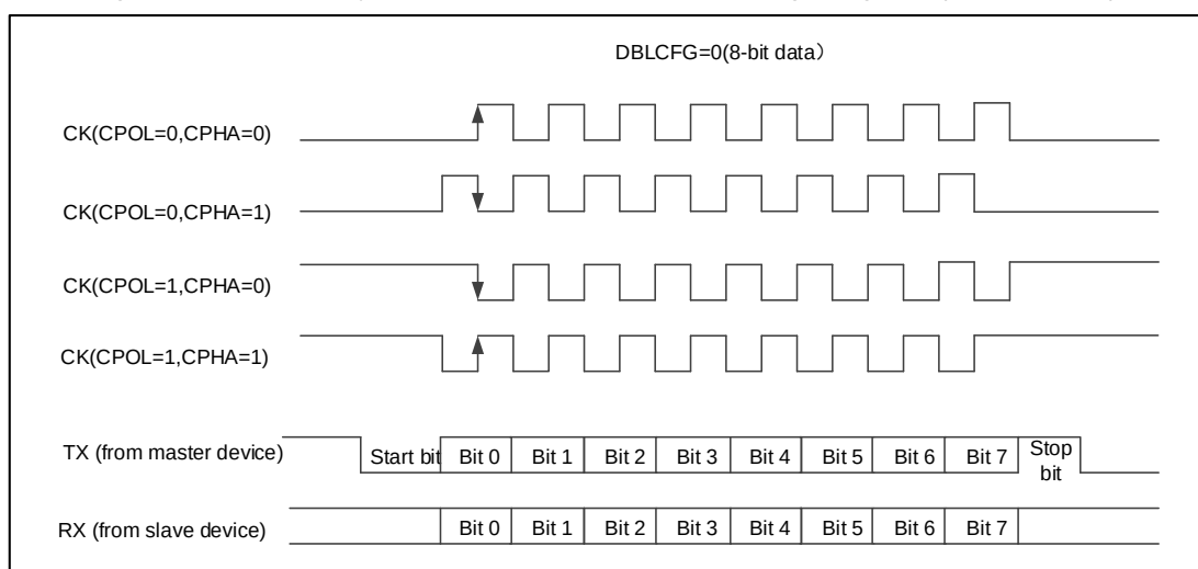
Figure 65 USART Synchronous Transmission Timing Diagram (DBLCFG=0)
