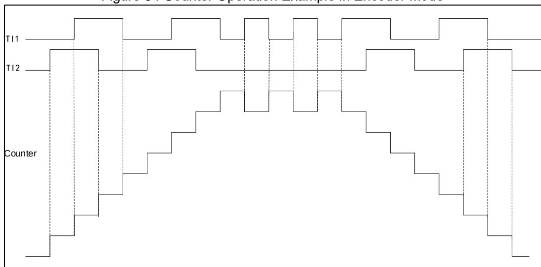
Figure 54 Counter Operation Example in Encoder Mode
