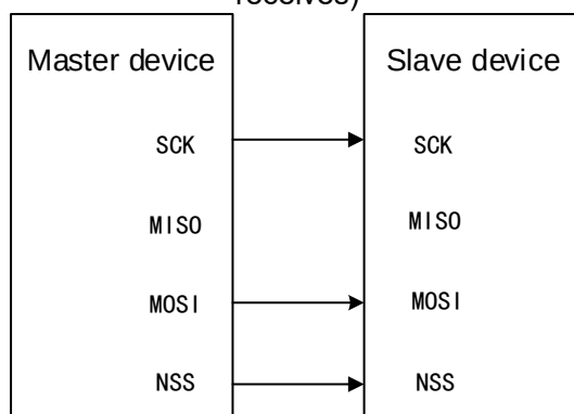
Figure 92 Connection in Simplex Mode (the master only transmits, while the slave receives)
