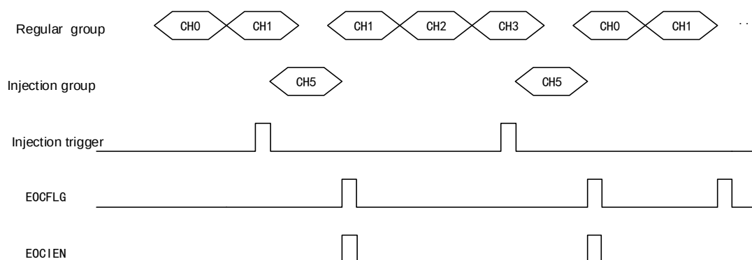
Figure 114 Trigger Injection Timing Diagram
